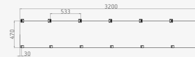
C4. Max. Design wind load: 5,3 kN/m^2
