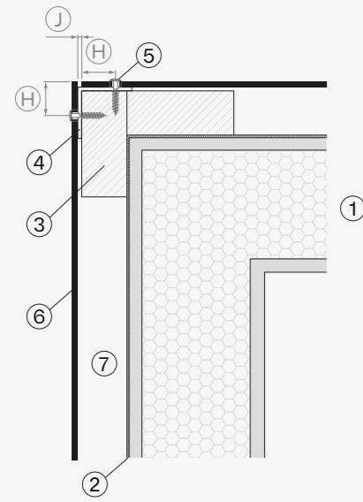
External corner
