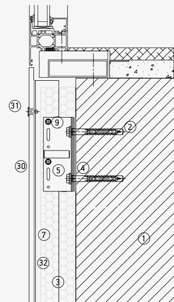
Window start
