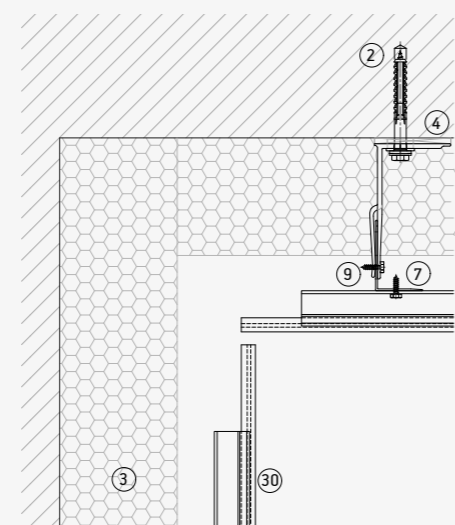
Internal Corner
