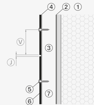
Horizontal joint
