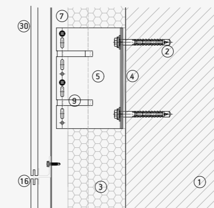
Horizontal joint
