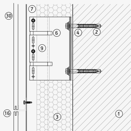
Horizontal joint
