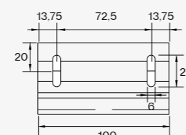
Intermediate clips with vertical holes
