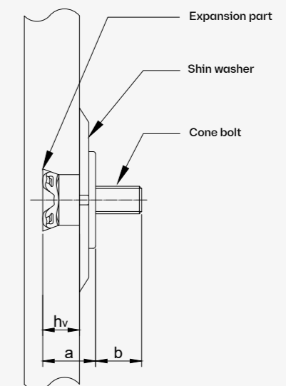
FISCHER FZP II Undercut anchor (DKT1.2)
