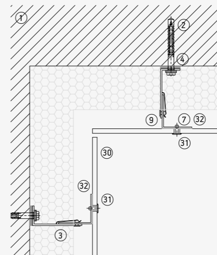
Interior corner
