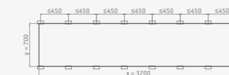
H1. Max. Design wind load: 1 kN/m 2
