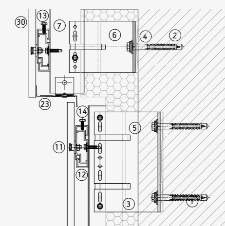
Joint option between profiles
