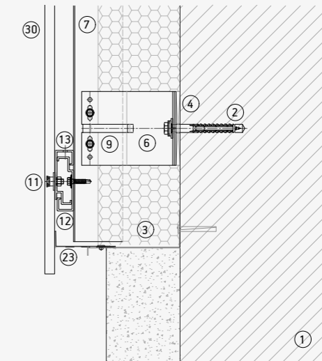
Joint option between profiles
