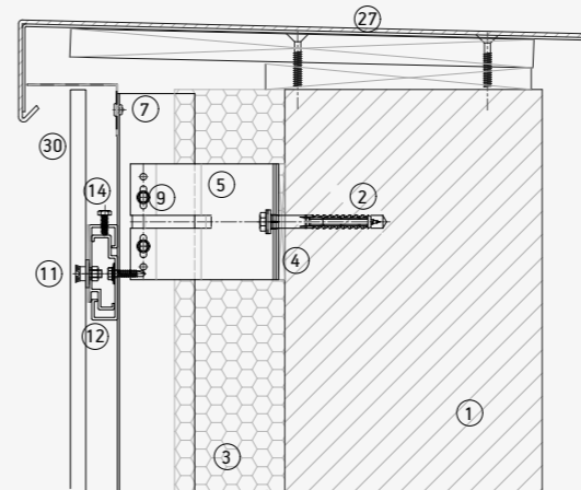
Upper detail
