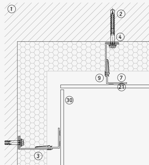
Internal Corner
