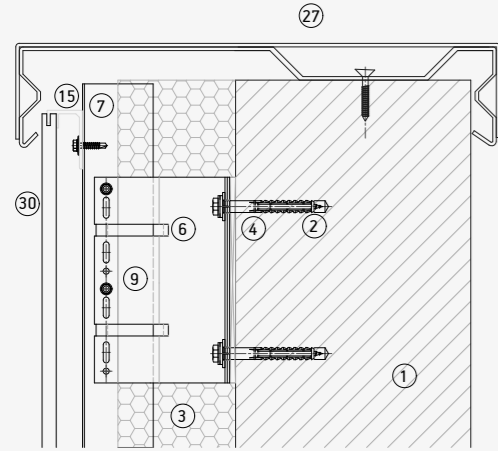
Upper detail
