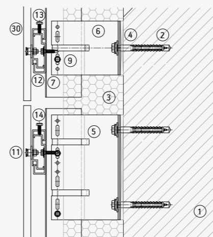
Horizontal joint
