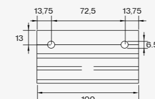
Intermediate clips with fixed drill holes
