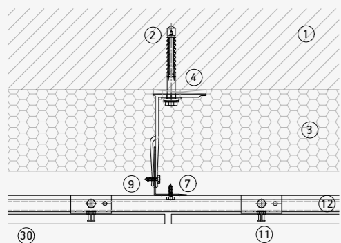
Vertical joint
