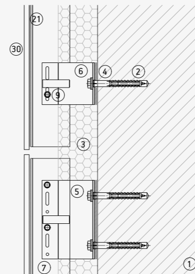
Horizontal joint
