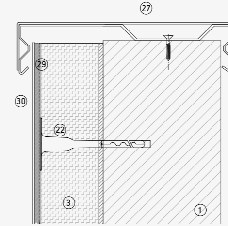
Upper detail
