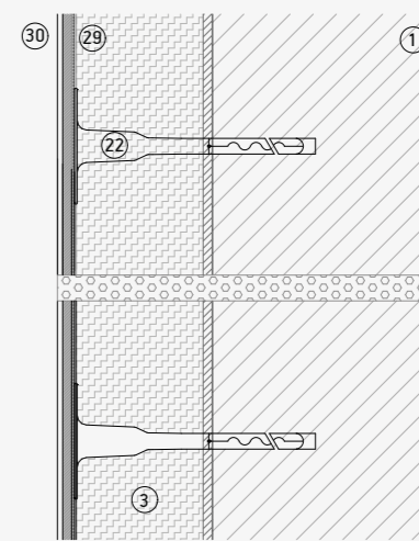
Horizontal profiles joint
