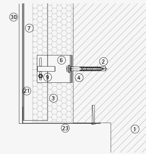
Bottom detail
