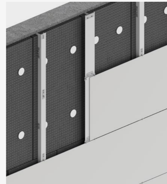
Bottom and middle clips
