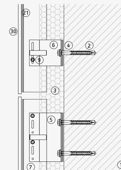
Joint between profiles
