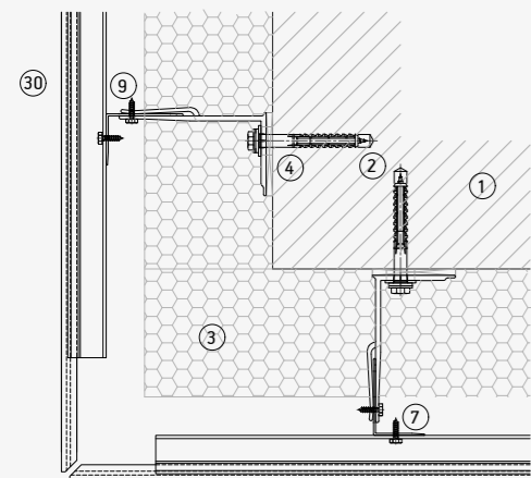
Mitered external corner
