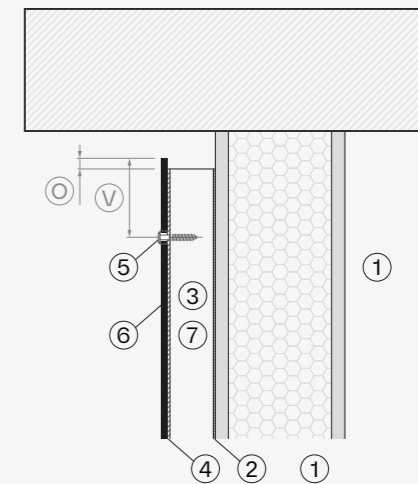
Upper detail
