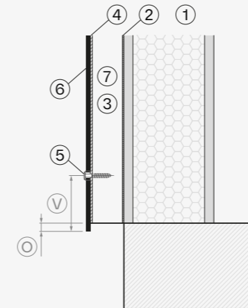
Bottom detail
