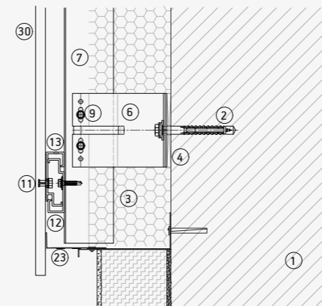
Bottom detail
