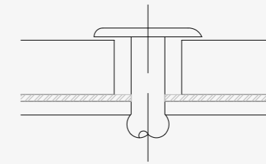
Sliding point Dekton 8 mm
