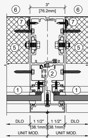
Vertical joint
