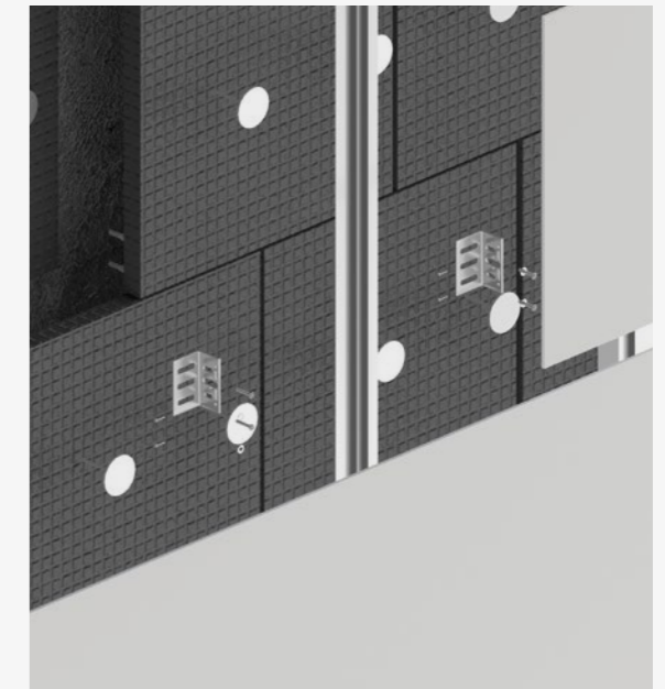
System detail
