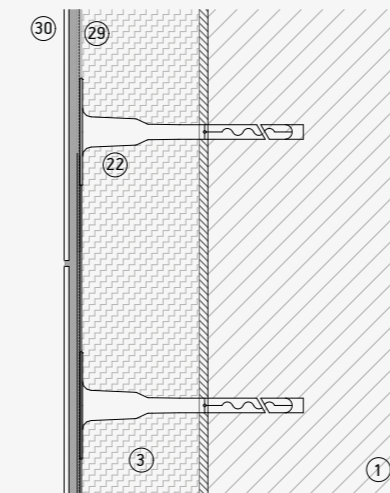
Horizontal joint
