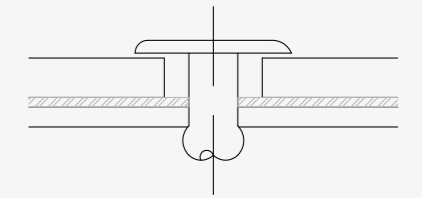
Sliding point Dekton 4 mm
