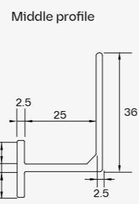
Cross-section DKT2.2
