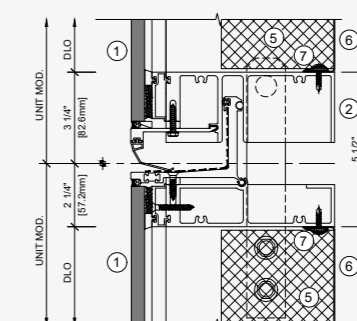
Horizontal joint
