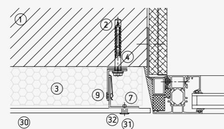
Window side
