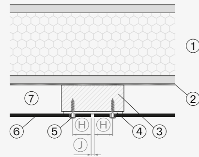
Vertical joint
