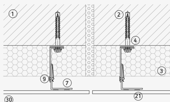
Vertical expansion joint
