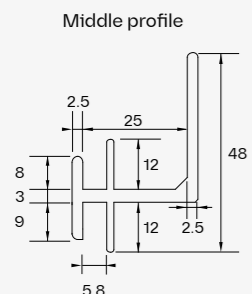
Cross-section DKT2.1
