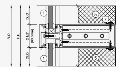
Horizontal joint
