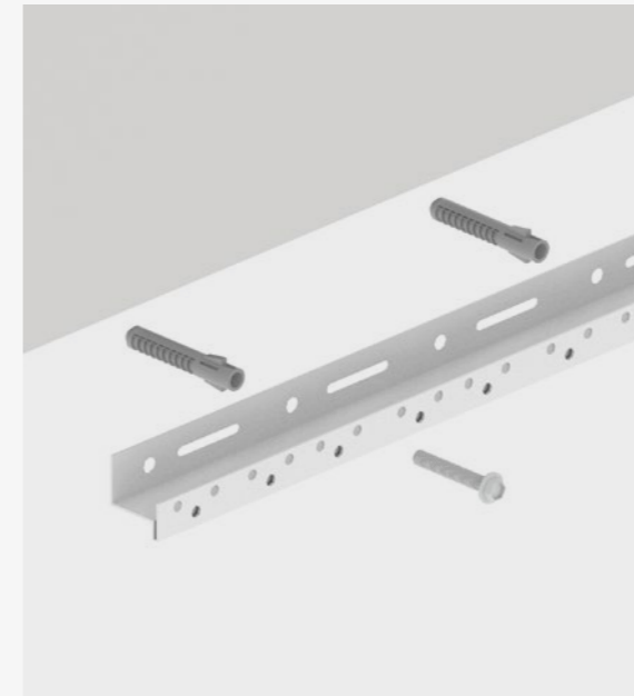
Starting profile
