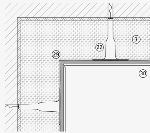
Internal Corner
