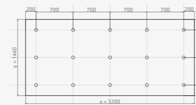
H2. Max. Design wind load: 3.0 kN/m 2
