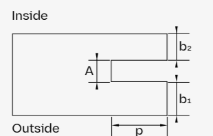
Geometry of the grooves
