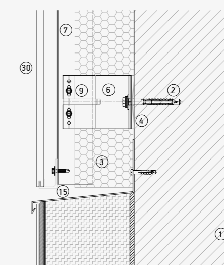
Bottom detail
