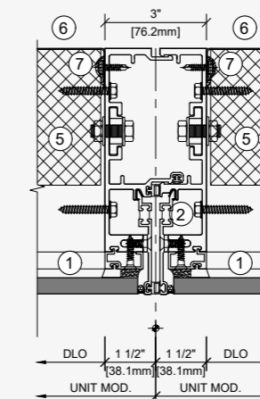
Vertical joint
