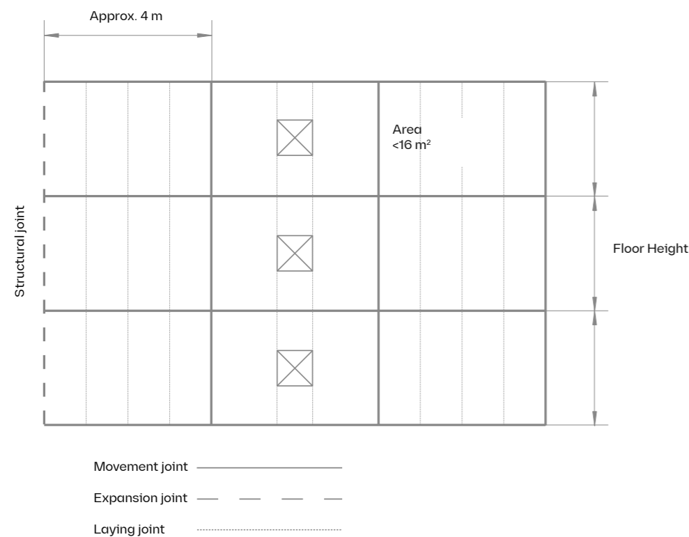
Diagram of joints on cladded facade
