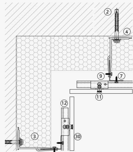
Internal Corner
