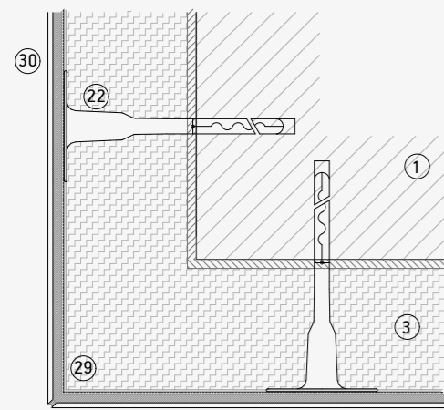
External corner
