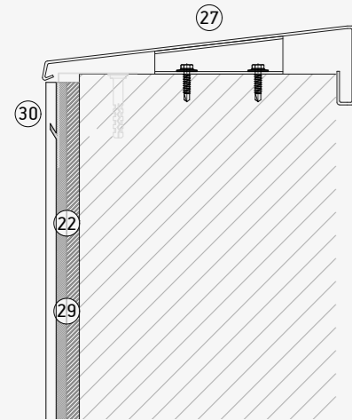
Upper detail
