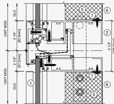
Horizontal joint
