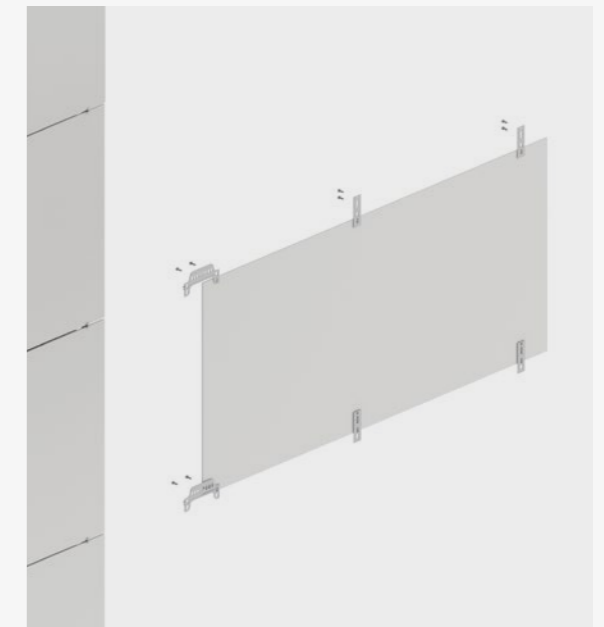
Middle clips
