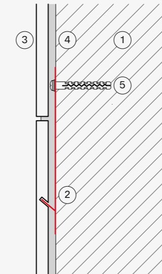
Cross section detail of the hidden safety fixing
