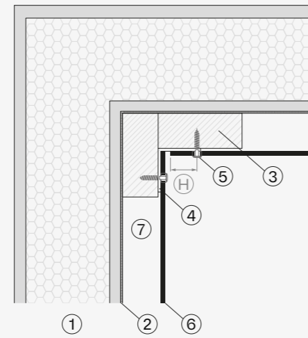
Internal corner
