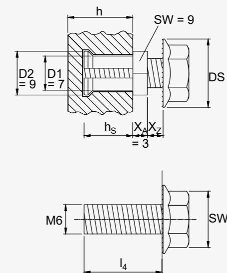
KEIL KH undercut anchor. Anchor sleeve and hexagonal screw (DKT1.1)
