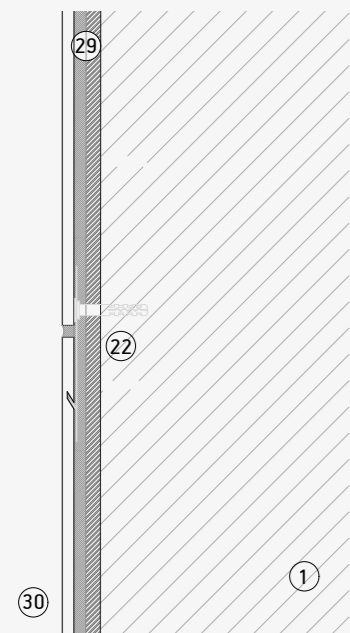
Horizontal joint
