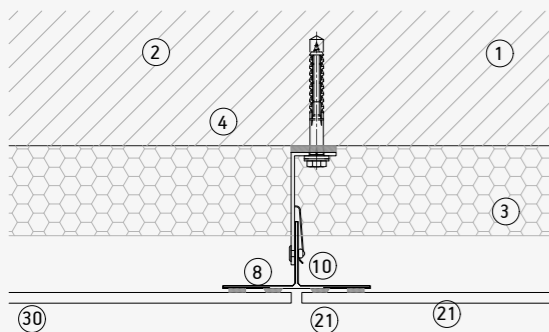
Vertical joint
