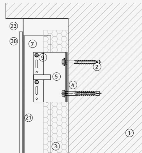
Upper detail
