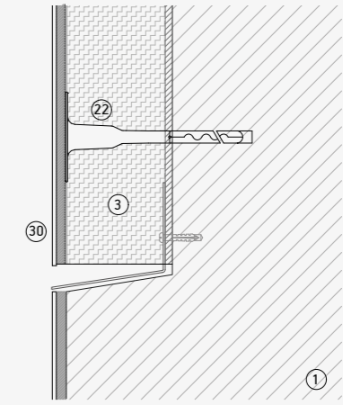
Bottom detail
